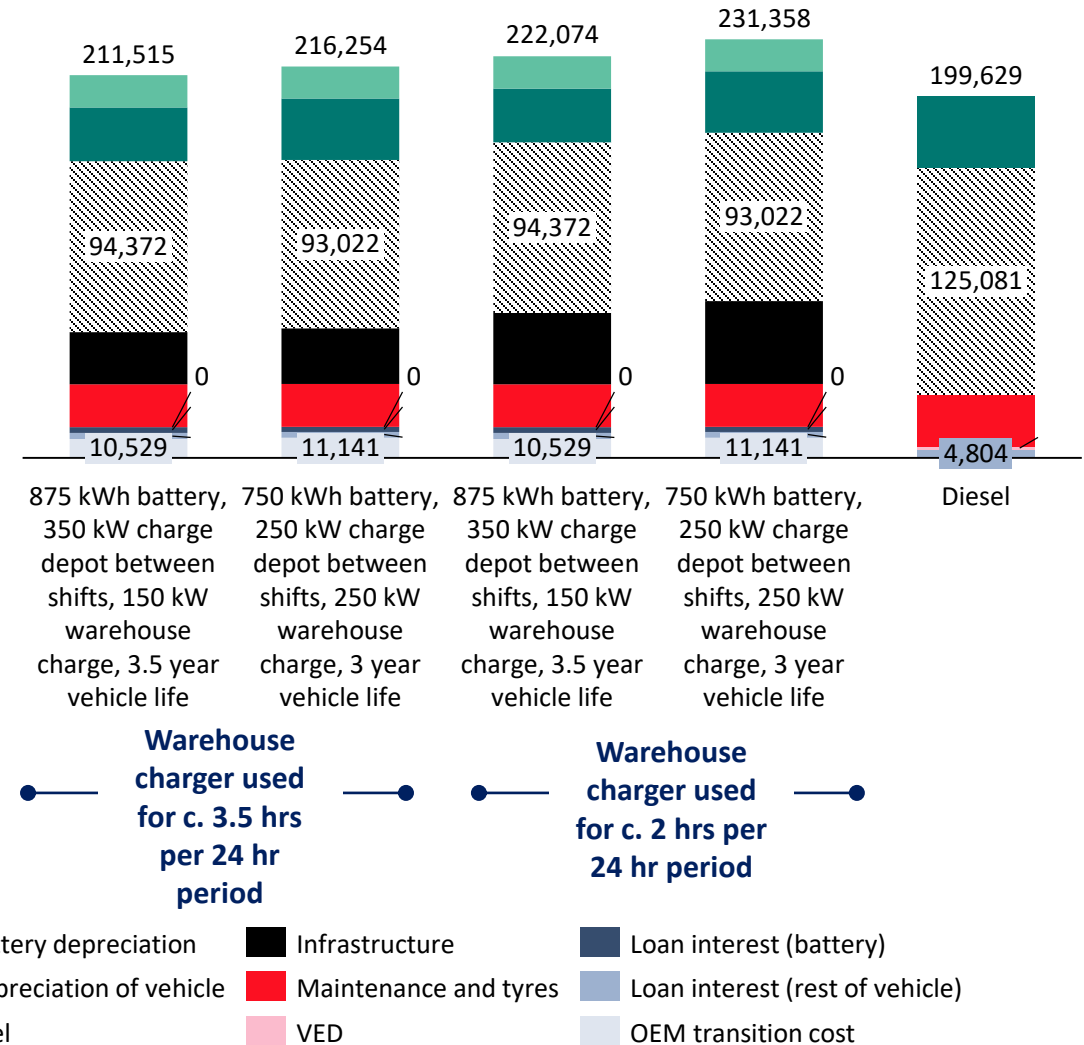
Annual TCO in £, 2030, for various charging options
