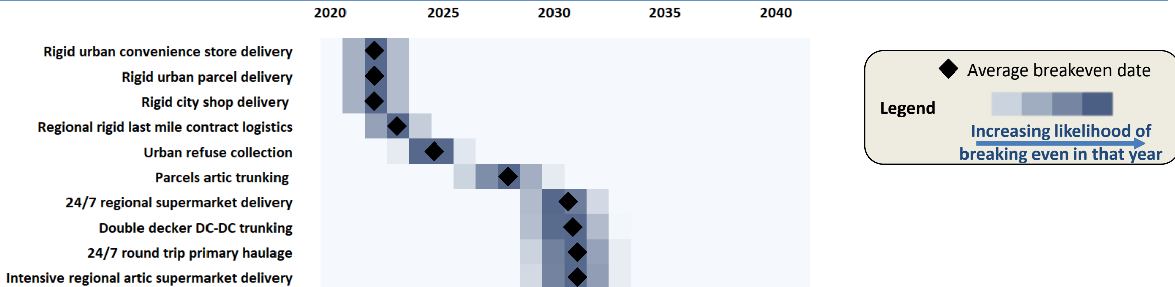
BEV-diesel TCO breakeven dates 1 for a broad sample of HGV use cases, without policy support and with conservative 2 assumptions on future improvements
