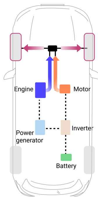
PHEV: parallel configuration
