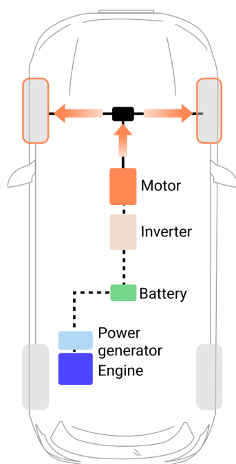
EREV: series configuration
