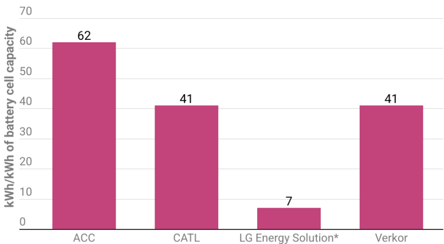
Energy consumption of battery gigafactories in Europe
